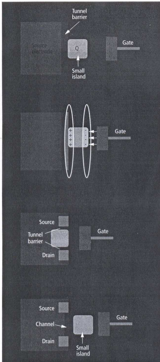
[5] The basic element in a quantum-dot transistor is called a single-electron box. The dot is a small conducting island separated by a tunnel barrier from a source electrode [top]. A positive voltage on the gate electrode polarizes the charges on the island (though the net charge may be zero), increasing the likelihood that an electron will tunnel between the source and the island [second from top].
